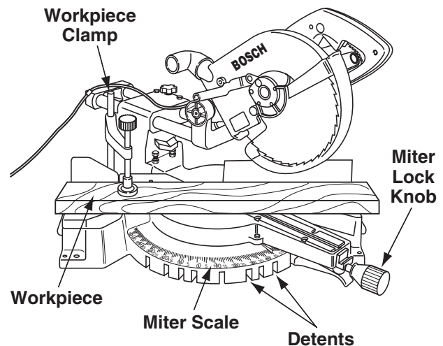
Figure 29. Miter Cut
