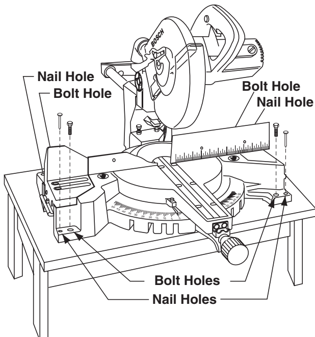
Figure 15. Workbench Mounting
