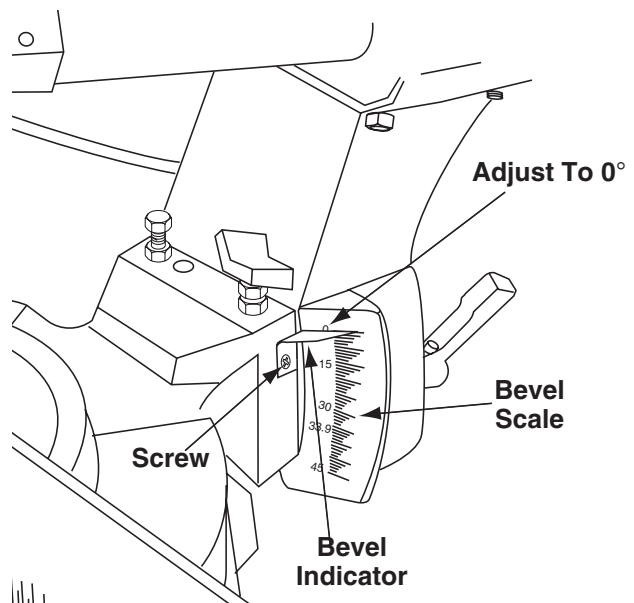
Figure 7. Bevel Indicator
