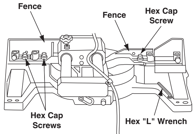
Figure 11. Fence Adjustment
